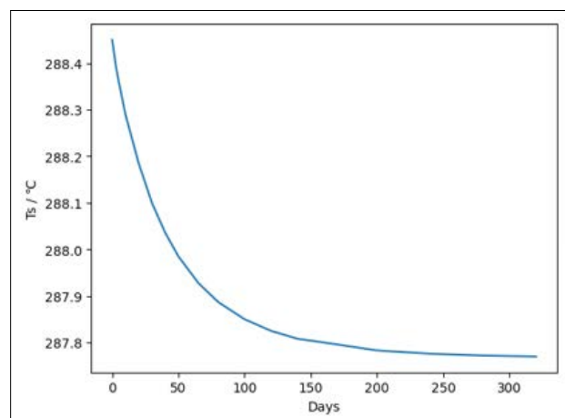
Figure 3: Surface Temperature Time Course after O 3 Increase
