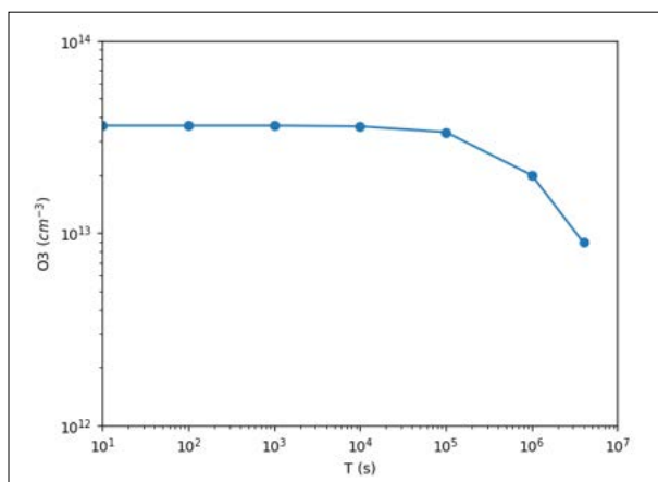
Figure 2: Change in O 3 Concentration after O 3 Injection
