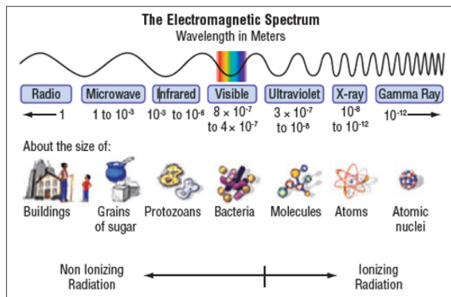
Figure 6: The Electromagnetic Spectrum of Radiation Waves (Source: NASA)
