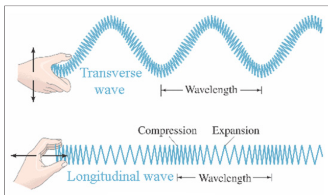
Figure 2: Illustration of Transverse versus Longitudinal Wave (Source: Scalar Wave Driven Energy Application book by Zohuri)
