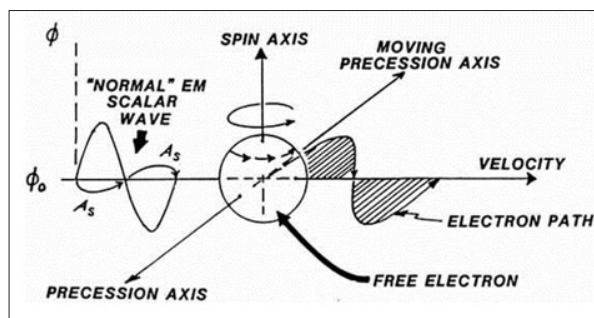
Figure 11: Illustration of Electron Path and Normal EM Scalar Wave
