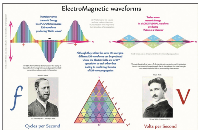
Figure 9: Electro-Magnetic Wave (EMW)
