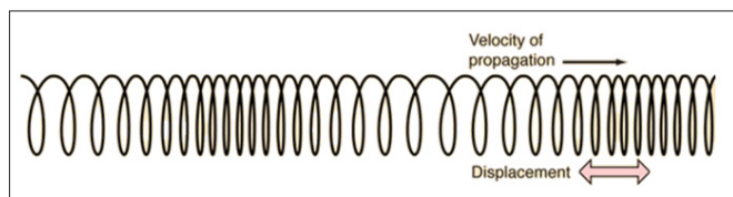
Figure 4: Depiction of a Longitudinal Wave
