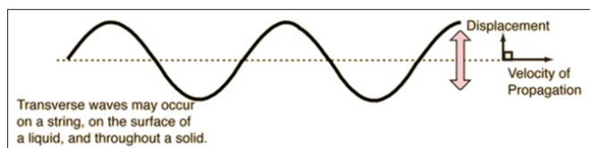
Figure 3: Depiction of a Transverse Wave
