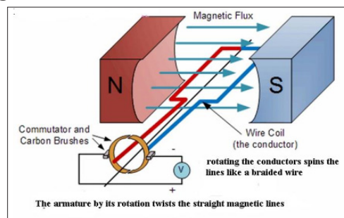
Figure 9: Electrical Generator
