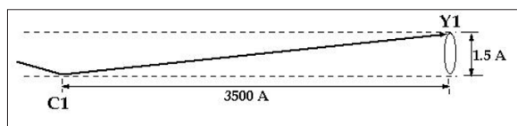
Figure 15: Half-Length of a Red Color Wave
