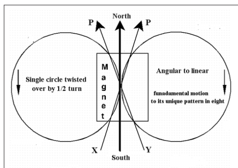
Figure 3: Birth of Magnetic. (Linear Movement).
