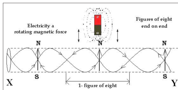
Figure 2: The Format and Pattern of a Rotating Magnetic Movement - known as Electricity.
