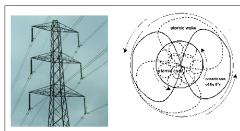
Figures 17 and 18: Magnetic Expansion
