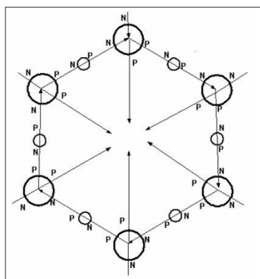
Figure 8: Water into Ice by Magnetic Polarities
