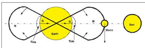
Figure 5: The Waters Rise on Both Sides of the Earth within the Figure Eight of Force. With Gravity Restraining it, as well as being a Factor in the Rising of the Waters
