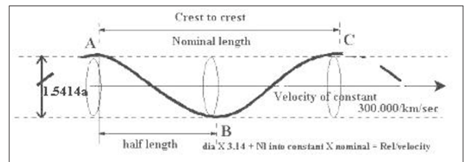
Figure 1: (So called) Waves by Two Velocities. The real velocity at the constant of 300.000-km/sec. Relative velocity; the one that is relative to the Angular Moment in it as the Speed for Nominal Distance.
