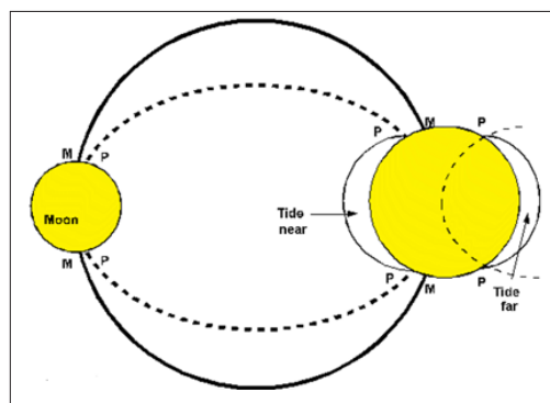
Figure 4: Waters Rise by Elongation
