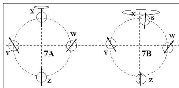
Figure 7: The Seasons by Precession just Short of One Turn of Orbit
