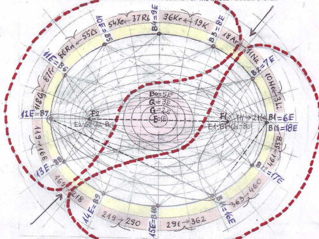
MATRIX REPRESENTATION OF ELLIPTIC CONIC SECTIONS WITH THEIR DANDELIN-SPHERES
