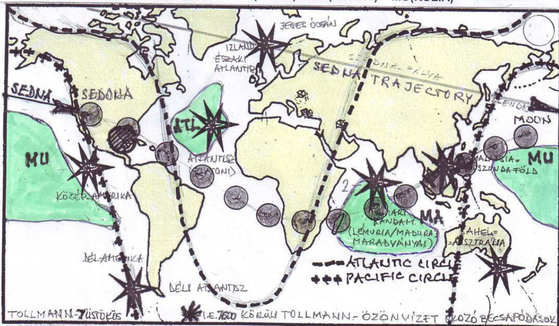
TRAJECTORY OF THE PLANETOID SEDNA WITH RESPECT TO THE FORMER CARAIBIAN (65 M YEARS AGO) AND TOLLMANN (7640 BC) CATASTROPHES
