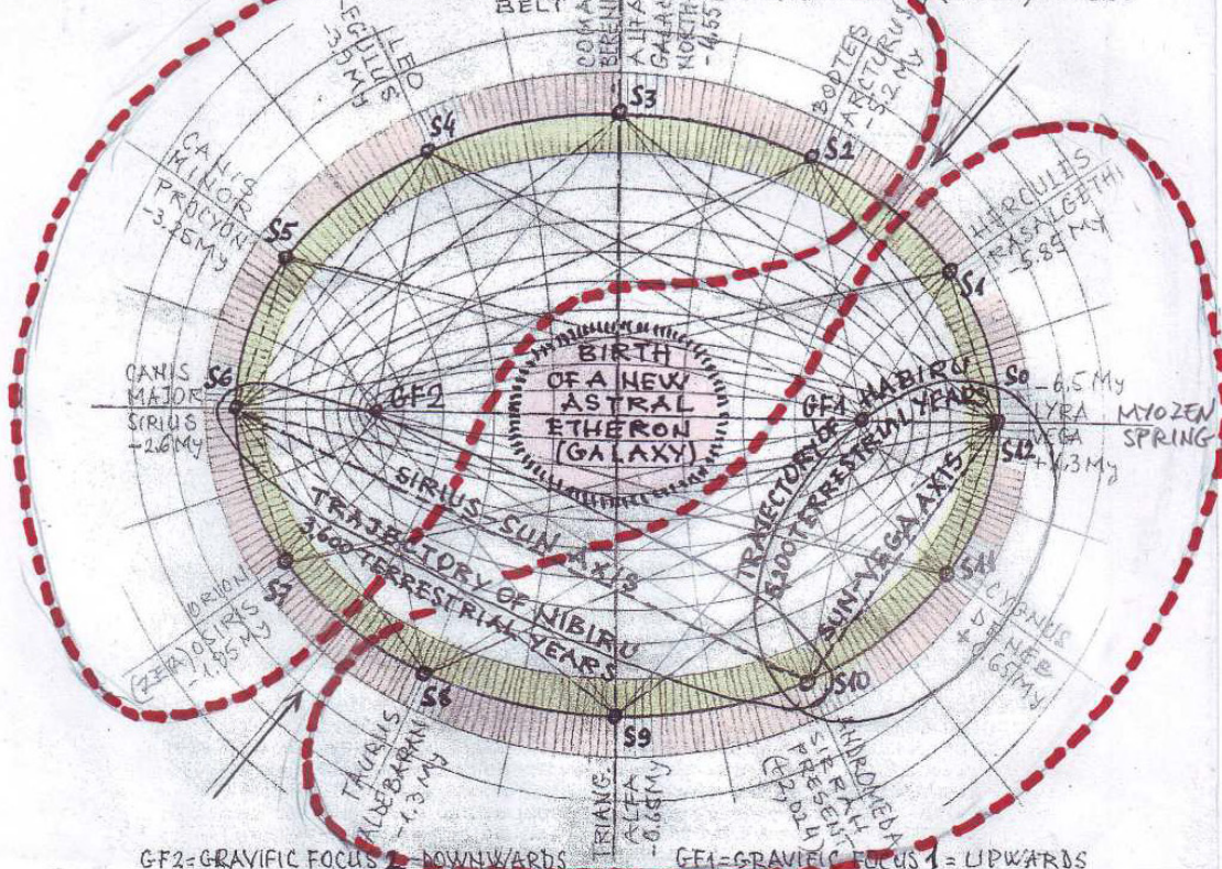
GF2=GRAVIFIC FOCUS 2 = DOWNWARDS
